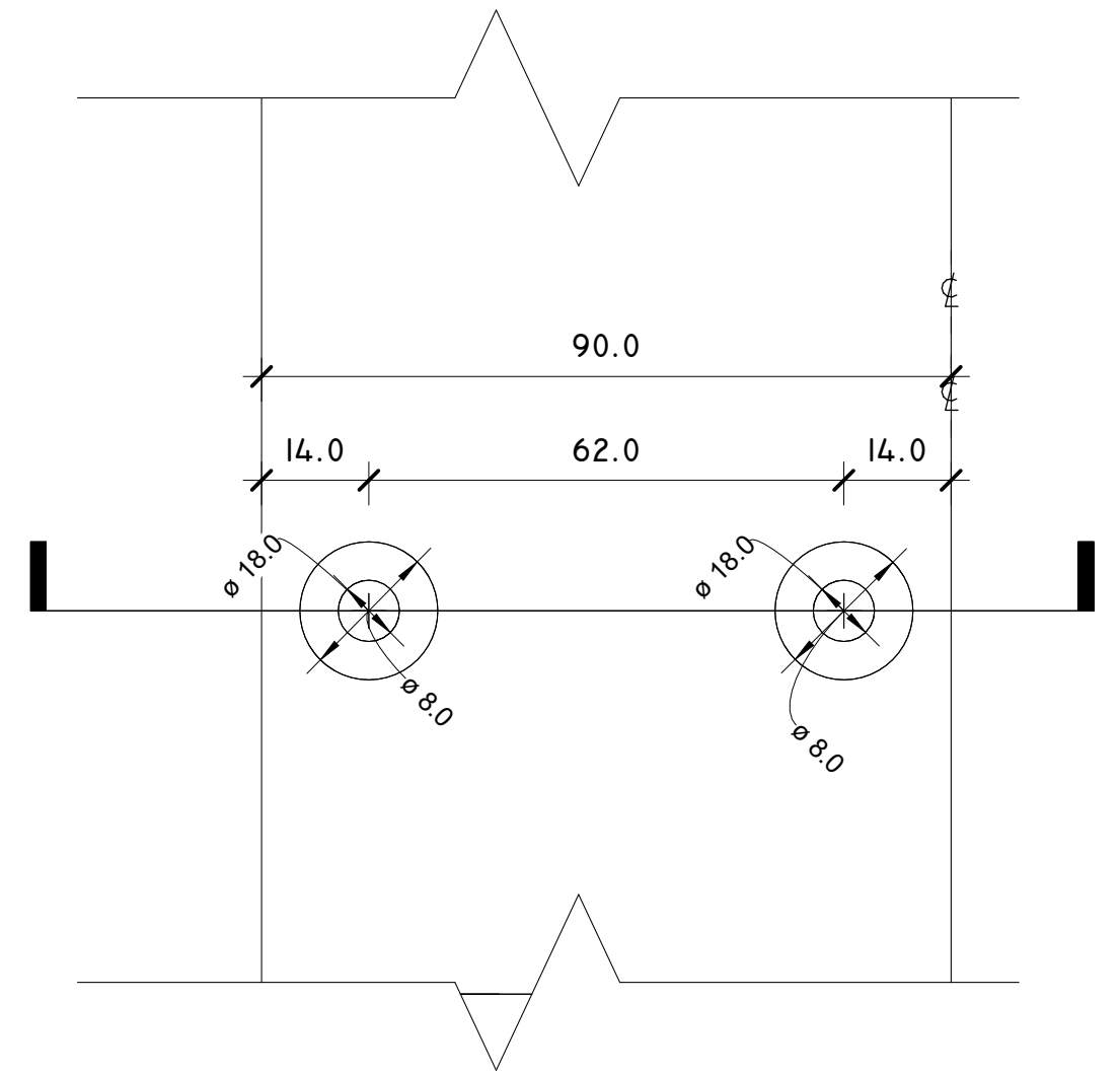
HOLE DIMENSIONS 1:1@A3 FOR MET-THERM BATTEN
