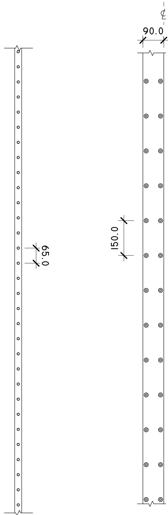
SIDE HOLE SPACING 1:10@A3 FOR MET-THERM BATTEN
