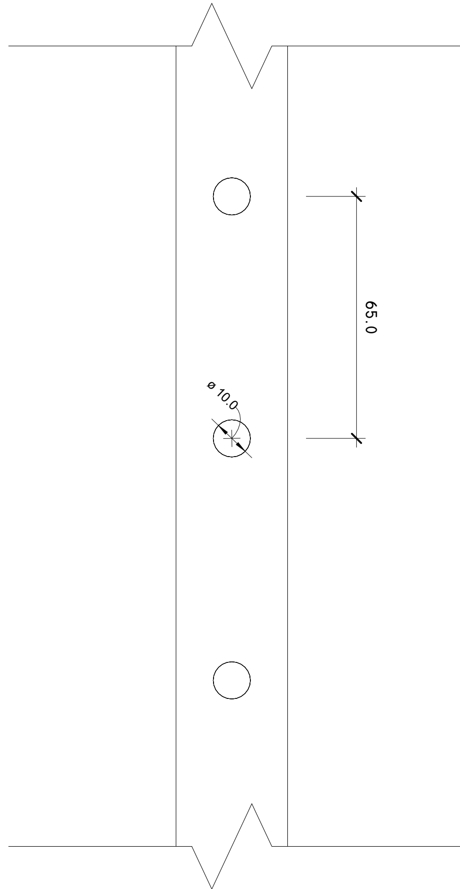
SIDE HOLE DIMENSIONS 1:1@A3 FOR MET-THERM BATTEN
