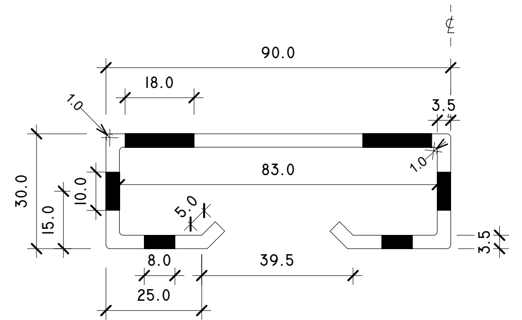
CROSS SECTION 1:1@A3
