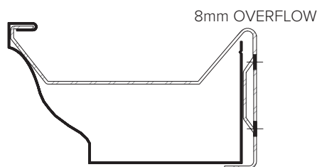
INTERNAL BRACKET
